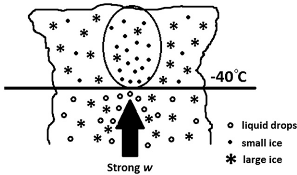
FIG. 6. Conceptual illustration of small, homogeneously nucleated ice particles (circled) being lofted above the -40^{\circ}\text{C} level by a strong thunderstorm updraft. These recently frozen ice particles suggest that supercooled water may exist below the -40^{\circ}\text{C} level.
