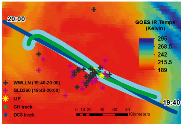
FIG. 9. GRIP aircraft tracks and WLLN/GLD360 lightning flashes between 1940 and 2000 UTC overlaid on 1945 UTC GOES IR imagery of Karl. The gold stars designate the location of the GH when LIP detected lightning flashes. A 10-km buffer (light blue) is placed along the GH flight track to highlight WLLN and GLD360 flashes near the aircraft.
