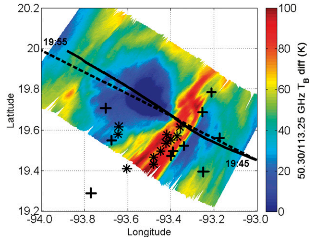
FIG. 10. The T_B differences between the 50.30- and 113.25-GHz channels of HAMSr from 1945 to 1955 UTC. Large T_B differences (red) in the southeast eyewall indicate regions where greater ice scattering, and thus deep convection, are occurring. WLLN [asterisk (*)] and GLD360 [plus (+)] flashes from 1945 to 1955 UTC, as well as GH (solid) and DC-8 (dashed) flight tracks, are overlaid for reference.
