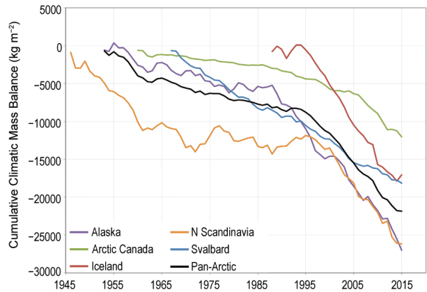
FIG. 5.15. Cumulative B_{\text{clim}} ( \text{kg m}^{-2} ) for glaciers in five regions of the Arctic, and for the Arctic as a whole (Pan-Arctic). Average balances are calculated for glaciers monitored in each region by summing annual averages for the period of record. Note that monitoring periods vary between regions and that the number and identity of glaciers monitored in a given region may vary between years.
