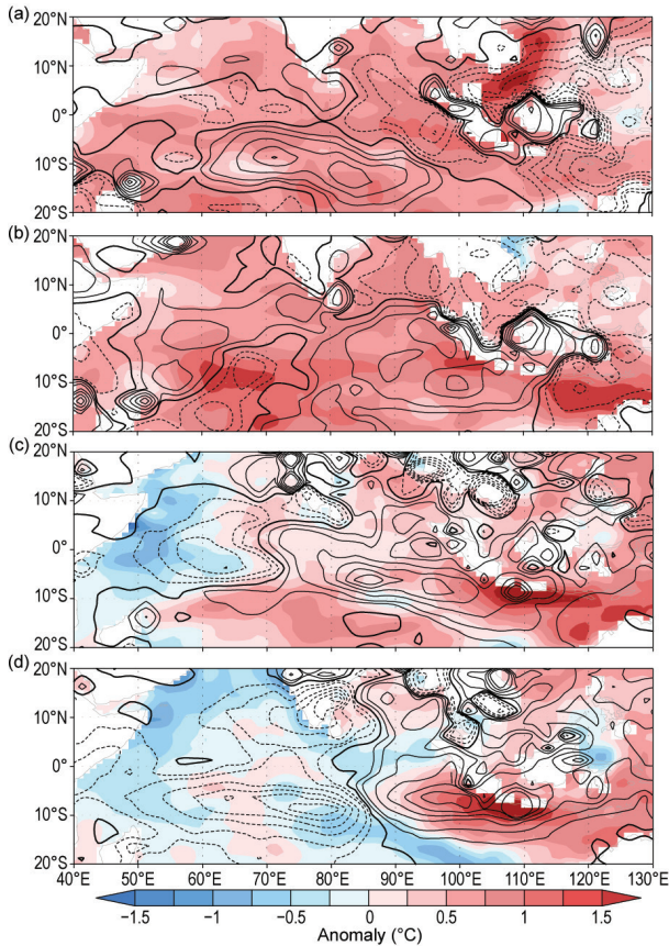
FIG. 4.42. SST (°C, colored scale) and precipitation (contour interval: 0, \pm 0.5 , \pm 1 , \pm 2 , \pm 3 , \pm 4 , and \pm 5 mm day -1 . Solid/dashed lines denote positive/negative values, and thick solid lines indicate zero contour) anomalies during (a) Dec 2015–Feb 2016, (b) Mar–May 2016, (c) Jun–Aug 2016, and (d) Sep–Nov 2016. The anomalies were calculated relative to the climatology over the period 1982–2015. [Source: NCEP optimum interpolation SST (Reynolds et al. 2002) and monthly GPCP precipitation analysis ( http://precip.gsfc.nasa.gov ).]
