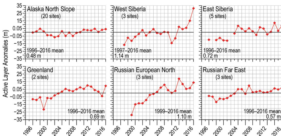
FIG. 5.25. Long-term ALT change (m, relative to average value for period of observations) in six different Arctic regions as observed by the Circumpolar Active Layer Monitoring program. Thaw depth measurements are made at the end of the thawing season. Only sites with at least 15 years of observations are shown.
