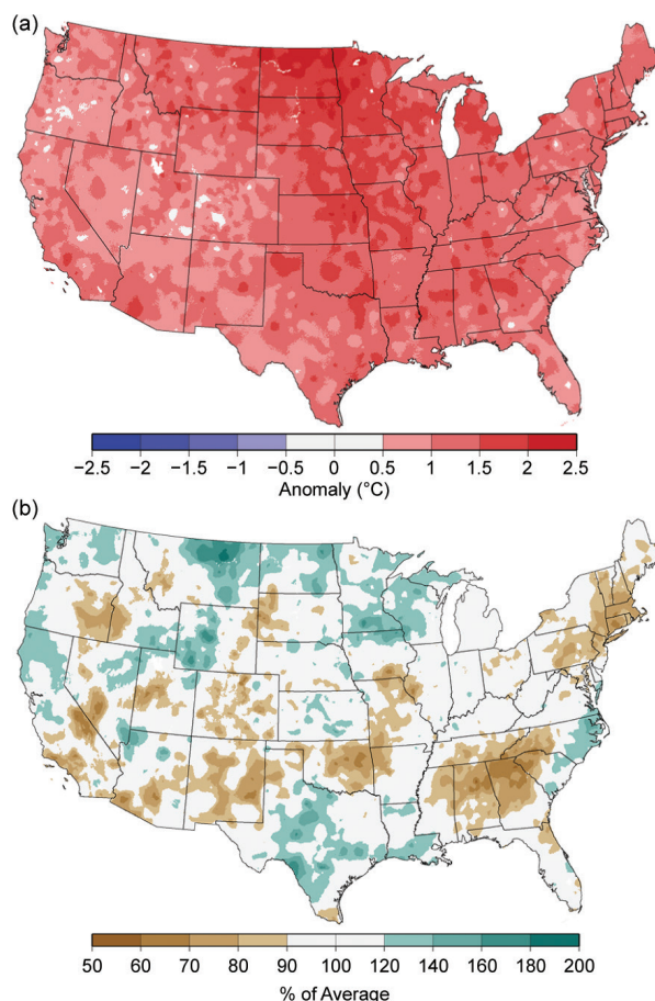
FIG. 7.4. (a) Annual average temperature anomalies (°C; 1981–2010 base period) and (b) % of average annual total precipitation in the contiguous United States for 2016. (Source: NOAA/NCEI.)
