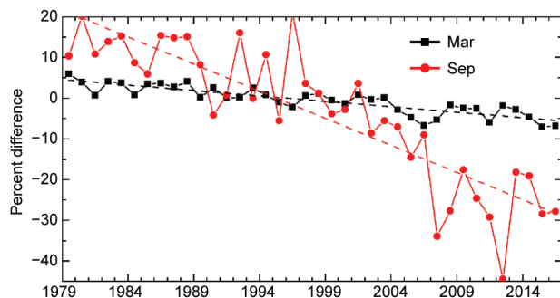
FIG. 5.5. Time series of ice extent anomalies (% relative to 1981–2010 averages) in Mar (maximum ice extent) and Sep (minimum ice extent). The black and red lines are least squares linear regression lines. The slopes of these lines indicate ice losses of 2.7% and 13.3% decade -1 in Mar and Sep, respectively. Both trends are significant at the 99% confidence level.
