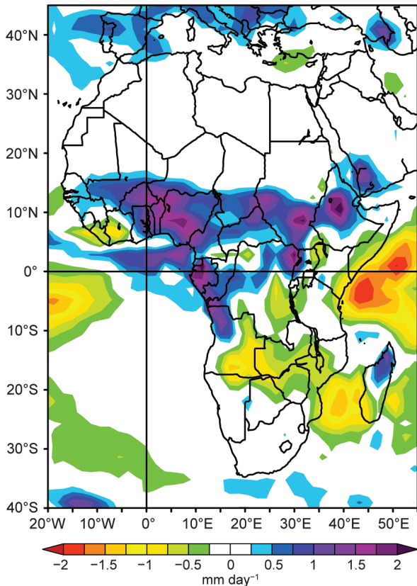
FIG. 7.17. Annual 2016 rainfall anomalies (mm day -1 ; 1981–2010 base period) over Africa. (Source: NOAA/NCEP.)
