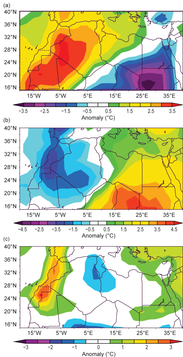
FIG. 7.18. Northern Africa 2016 surface air temperature anomalies (°C; 1981–2010 base period) for (a) Jan, (b) Mar, and (c) Jul–Aug. (Source: NOAA/NCEP.)
