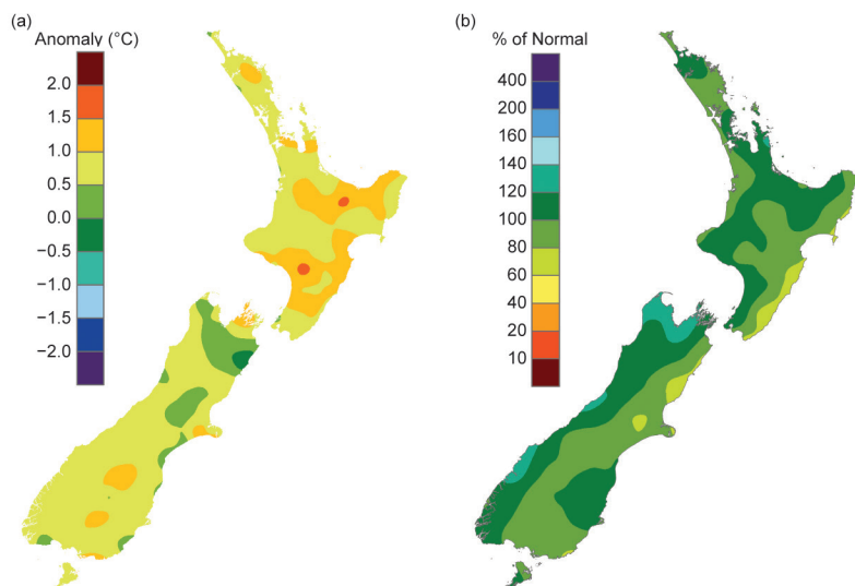
FIG. 7.61. (a) 2016 annual mean temperature anomaly (°C) and (b) 2016 annual total rainfall (%), relative to 1981–2010. (Source: NIWA.)
