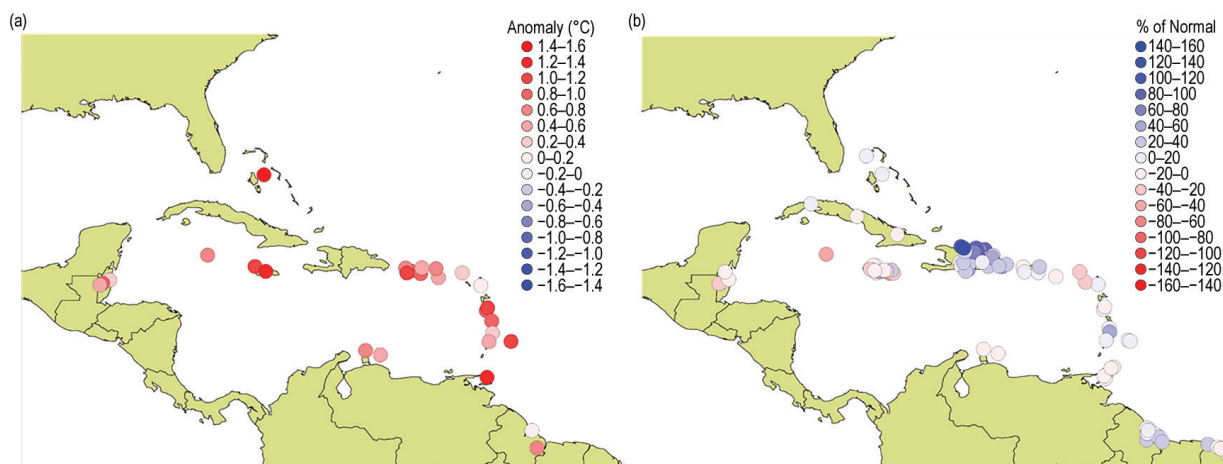
FIG. 7.11. (a) Temperature anomalies (°C) and (b) precipitation anomalies (%) rainfall for 2016 across the Caribbean basin with respect to the 1981–2010 annual mean. (Source: Caribbean Institute for Meteorology and Hydrology.)
