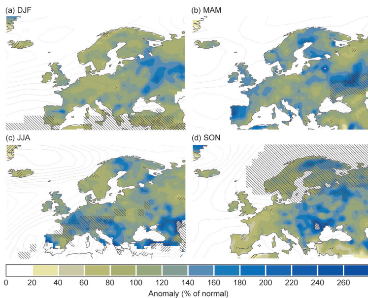
FIG. 7.38. Seasonal anomalies for 2016 (1981–2010 base period) of sea level pressure (hPa, contours) and seasonal precipitation anomalies (% shading) from NCAR–NCEP reanalysis for (a) DJF, (b) MAM, (c) JJA, and (d) SON. Left hatches indicate where the anomaly at sea level pressure is significant at the 5th or 95th percentile. Right hatches show the same conditions for seasonal precipitation. White areas have received either less than 20% of normal or below 15 mm seasonal precipitation. Negative sea level pressure anomalies are indicated by dashed contours. Black areas indicate regions where data have been inadvertently omitted from the figure. Please note the base period used here is different from that used in Fig. 7.37. (Source: NOAA/ESRL Physical Sciences Division, www.esrl.noaa.gov/psd .)
