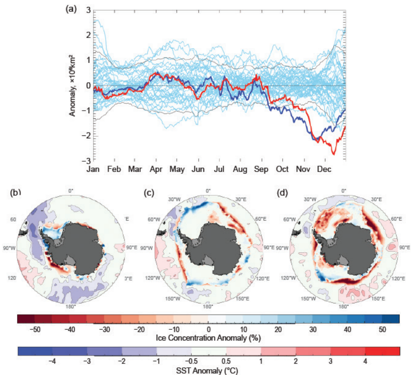
FIG. 6.8. (a) 2016 daily anomaly ( 10^6 km 2 ) of SH sea ice extent (red line) and area (dark blue line), from the 1981–2010 mean. Thin blue lines represent the historical daily values of extent for 1979–2015, while the thin black lines represents \pm 2 std. dev. of extent. Sea ice concentration anomaly (%) for (b) Feb (c) Aug 2016 (d) Nov, (relative to 1981–2010 monthly means), along with monthly mean SST anomalies ( ^{\circ} C; Reynolds et al. 2002; Smith et al. 2008). Bell is Bellingshausen Sea.
