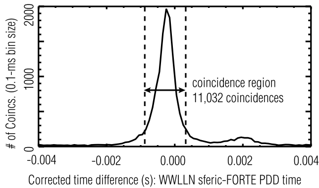
Figure 1. Time difference histogram of WWLLN-sferic time minus FORTE PDD trigger time, corrected for optical signal delay to satellite. Bin size is 0.0001 s. The peak occurs at approximately -250 \mu\text{s} , indicating that the PDD optical is triggered about 250 \mu\text{s} after WWLLN detects the sferic. The two vertical dashed lines indicate the timing cutoffs for coincident events ( -0.80 to 0.30 -ms timing difference). 11,032 events fall within the cutoff times.
